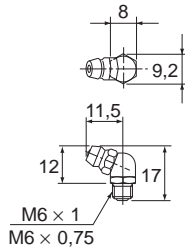
B-M6F (M6×0,75)
