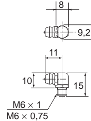
C-M6F (M6×0,75)
